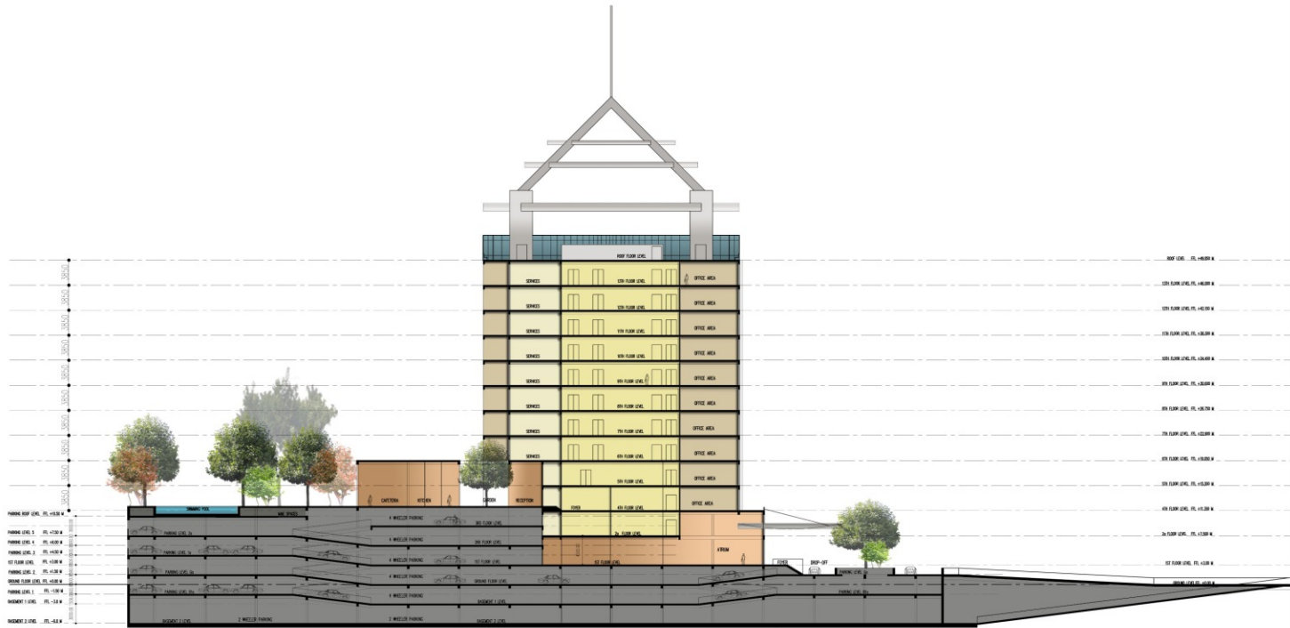
SCHEMATIC SECTION
