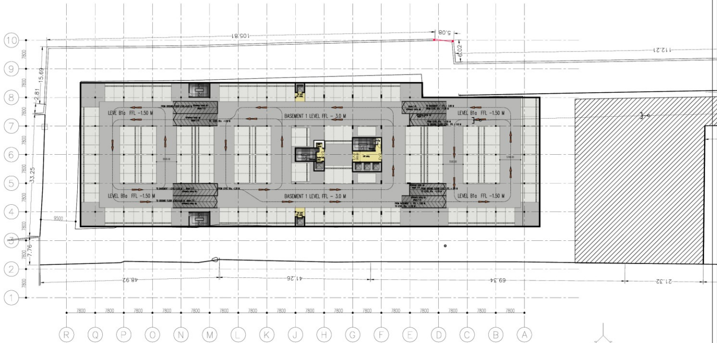
BASEMENT 1 PLAN
