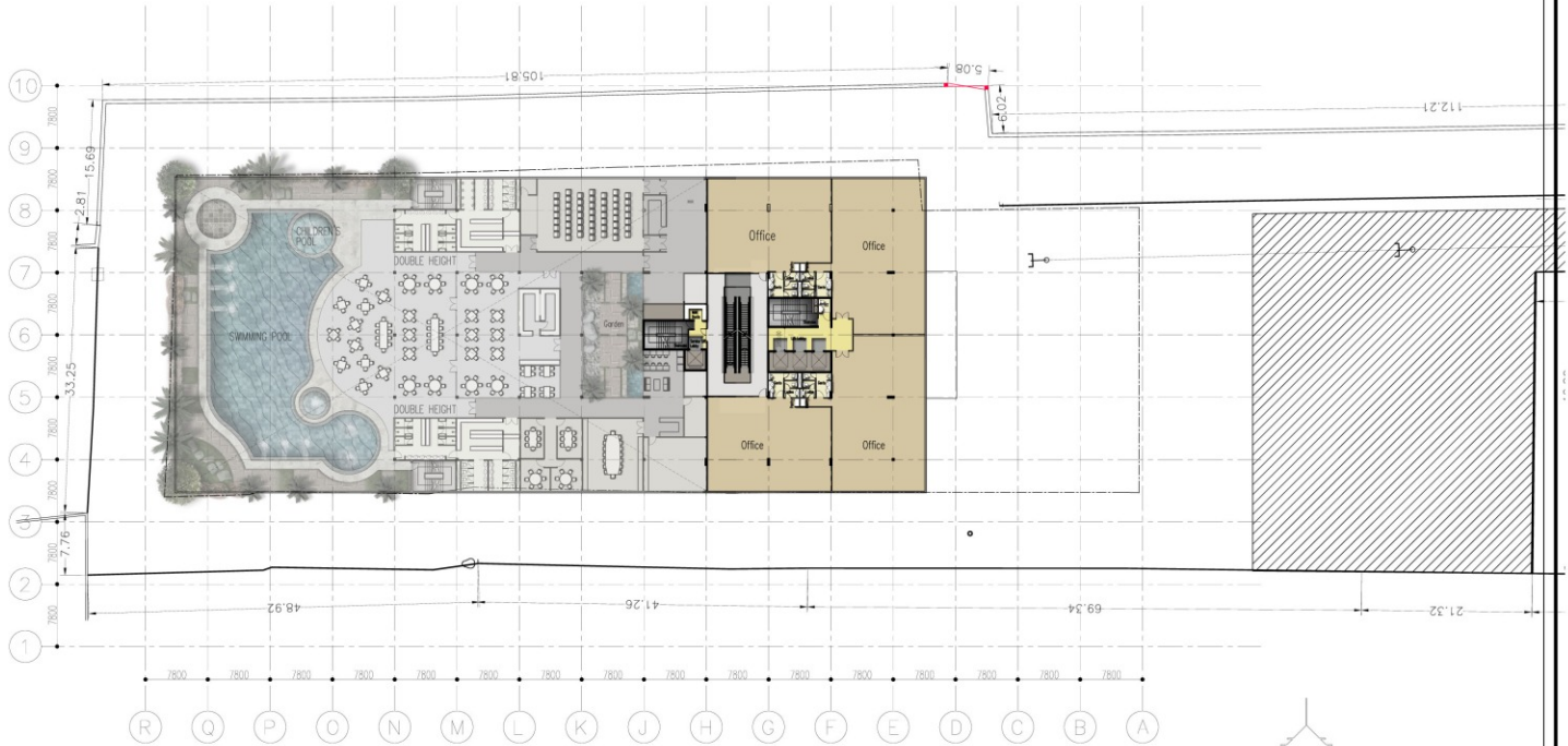
5TH STOREY PLAN
