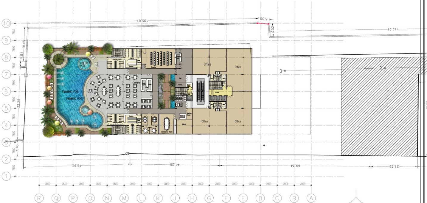
4TH STOREY PLAN
